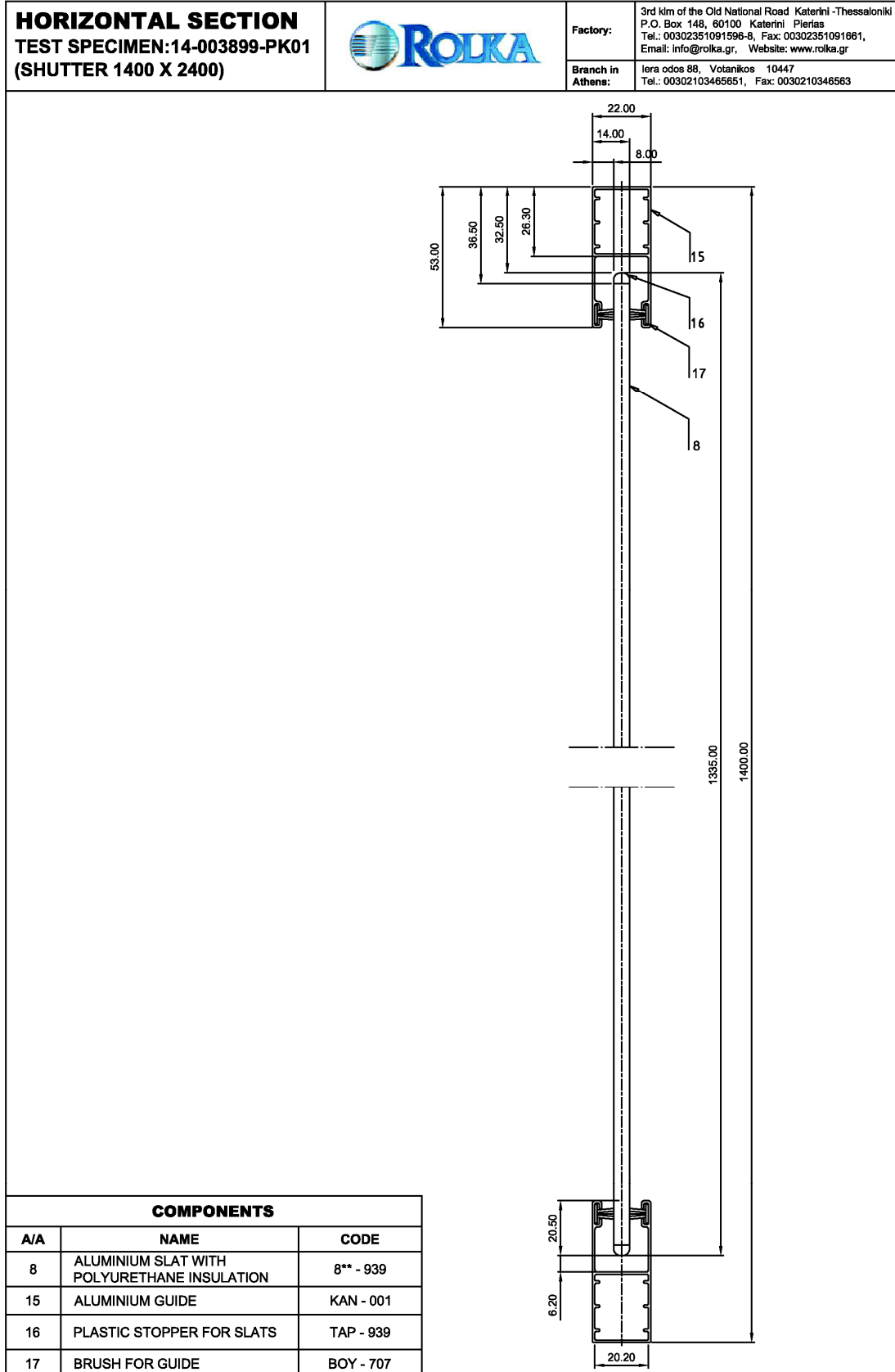
Figure 2 Horizontal section
