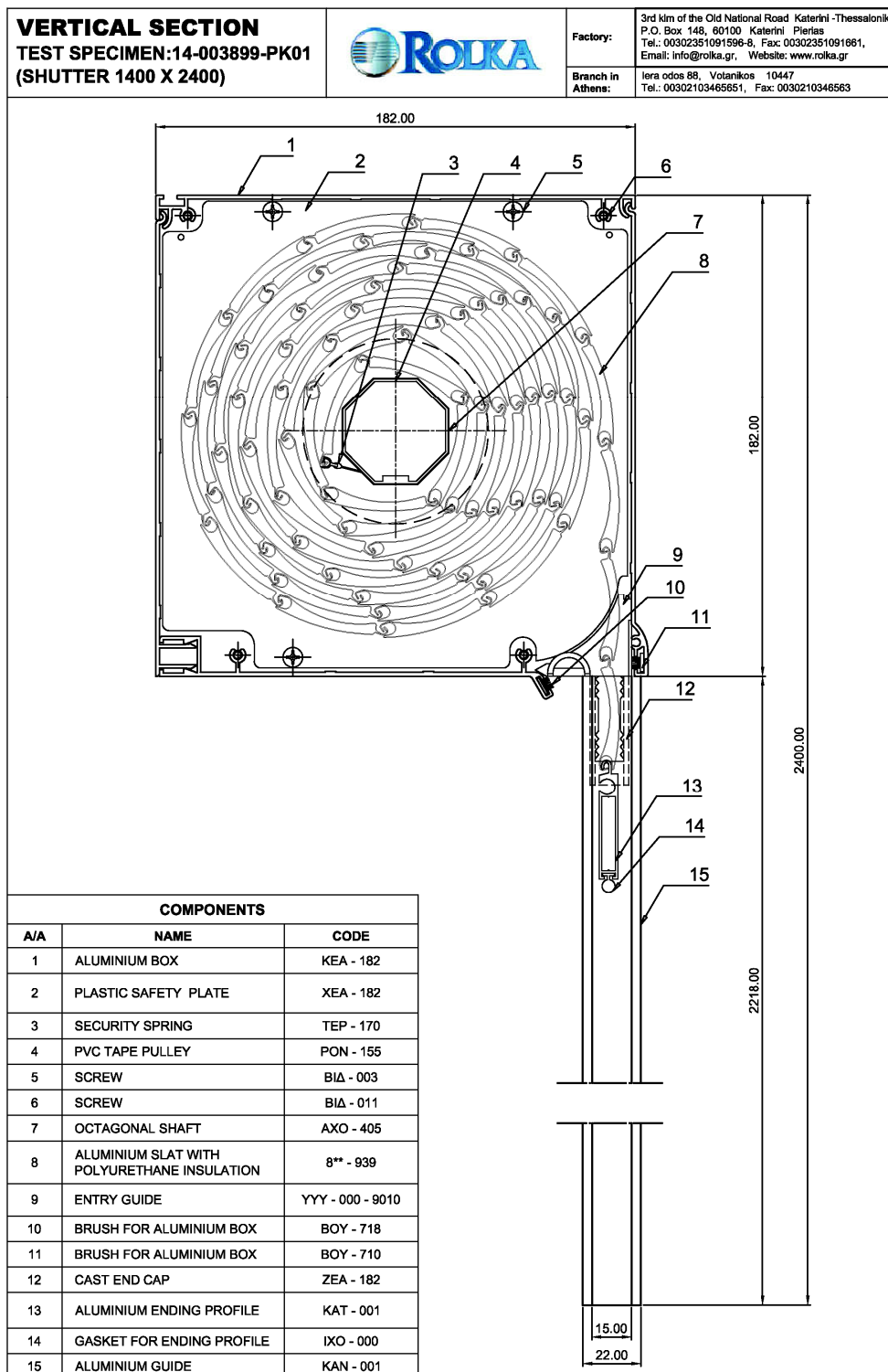
Figure 1 Vertical section
